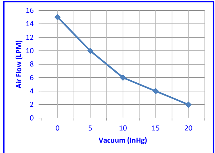
Vacuum Input Air Flow
