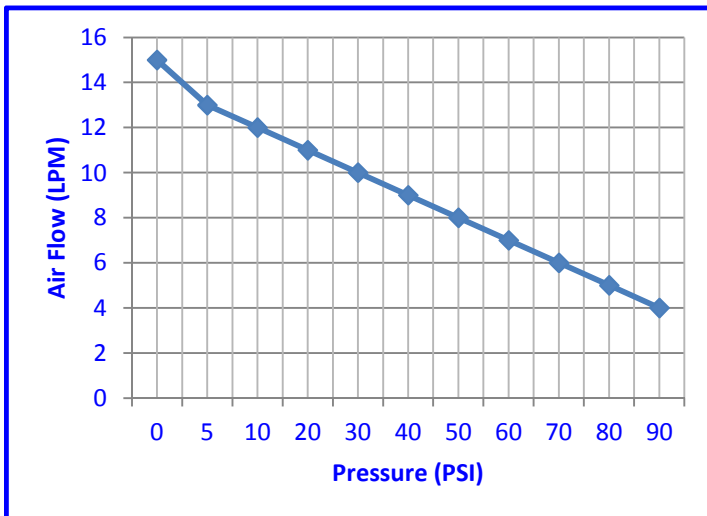
Pressure Output Air Flow
